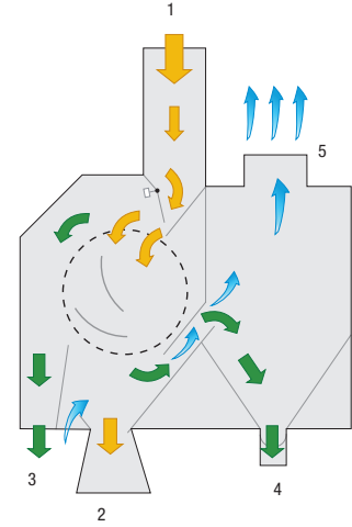
Drum Cleaner with Aspiration System
