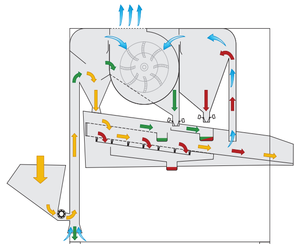
Working principle Seed Cleaner Type K 06
